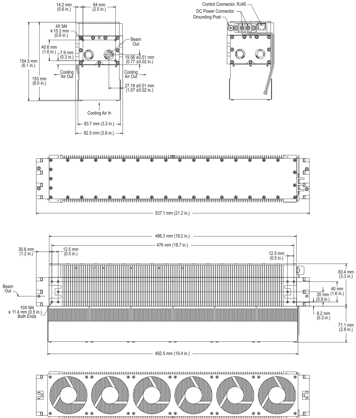
Figure 4-2. C-55 Air-Cooled Laser Dimensions
