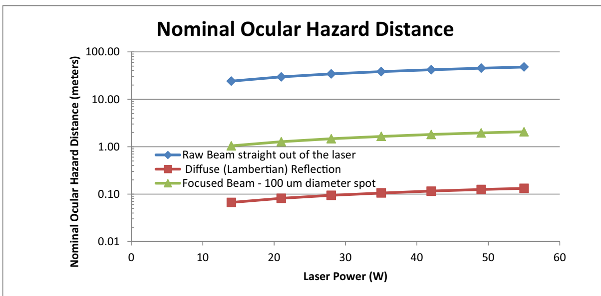
Figure 2-1. Nominal Ocular Hazard Distance (NOHD) for indicated conditions calculated per ANSI Z136.1-2007
