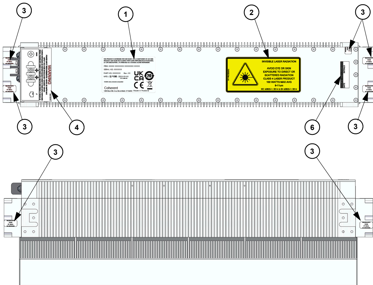
Figure 2-2. Location of Safety Labels (Sheet 1 of 2)
