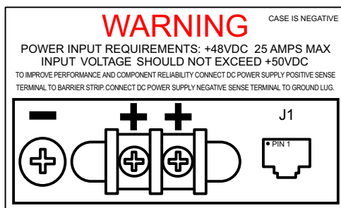
4. Voltage Warning Label
