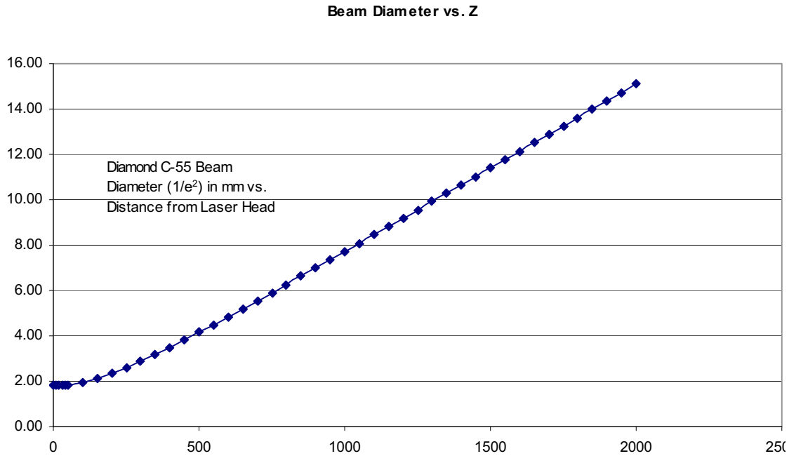
Figure 4-4. Beam Diameter vs. Distance From Laser Head
